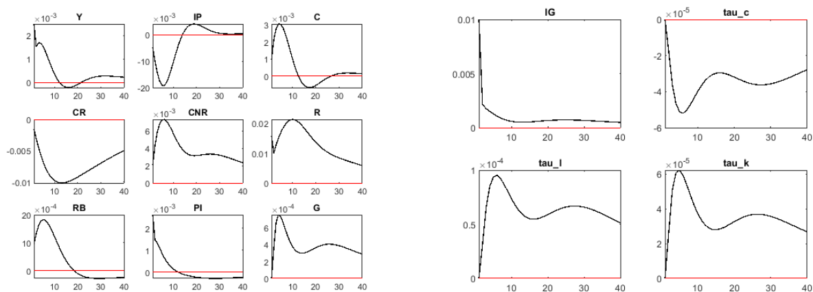
Figure 2: Orthogonalized shock to e_{IG} : augmentation des investissements publics
