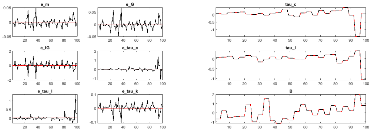
Figure 10: smoothed shocks/Historical and smoothed variables
