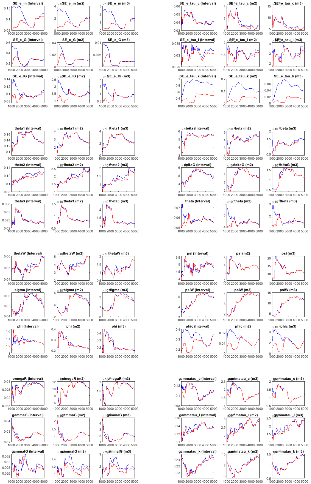
Figure 8: MCMC univariate convergence diagnostic (Brooks and Gelman, 1998)
