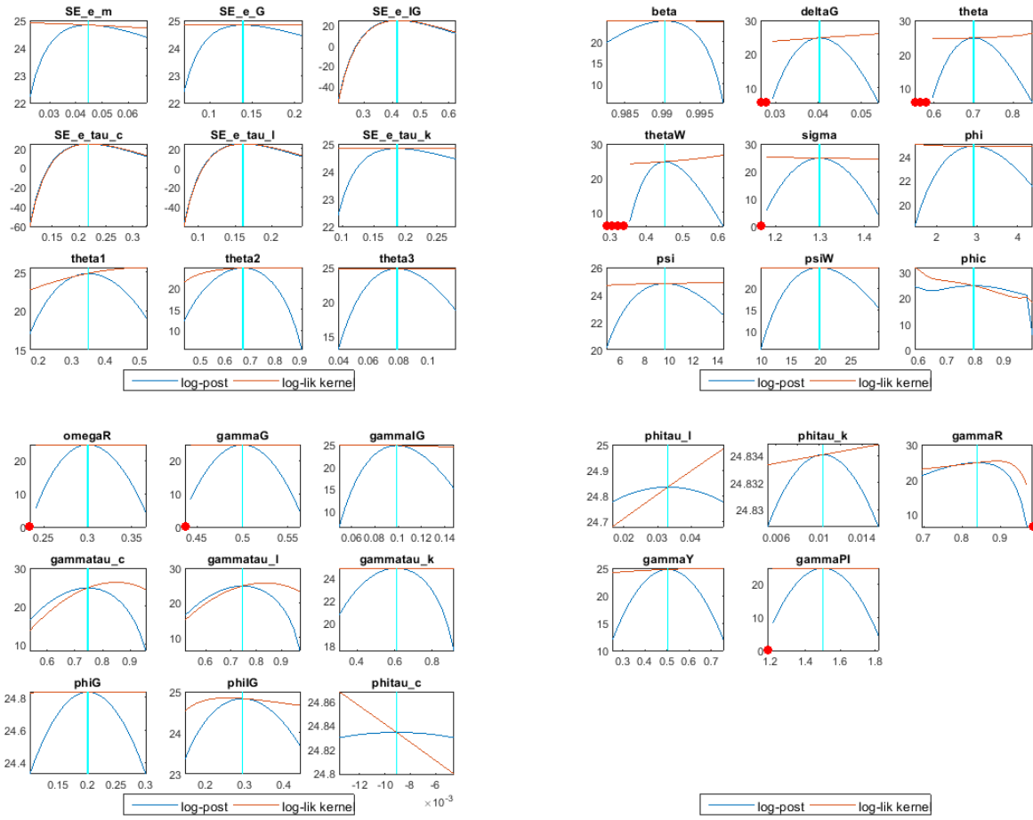
Figure 11: mode check plots
