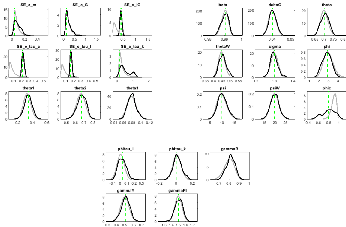
Figure 7: priors and posteriors distributions parameters
