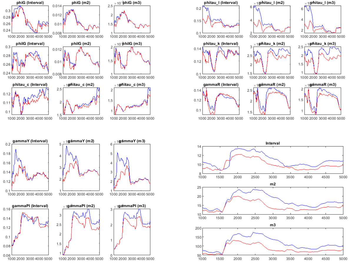
Figure 9: MCMC univariate convergence diagnostic (Brooks and Gelman, 1998)/Multivariate convergence diagnostic
